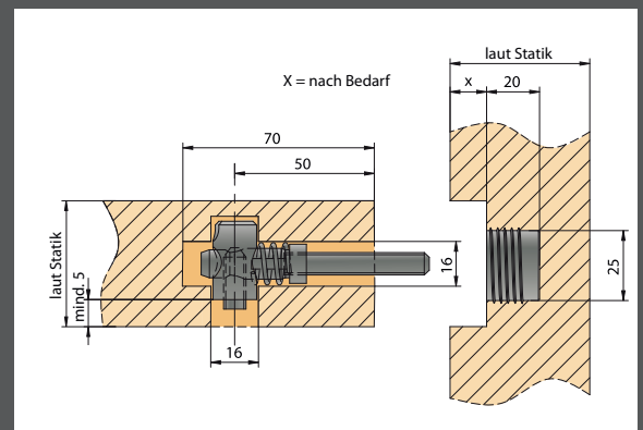
easy-con® M8-16-50
