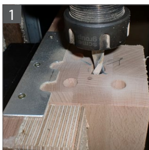
1 Bohren
